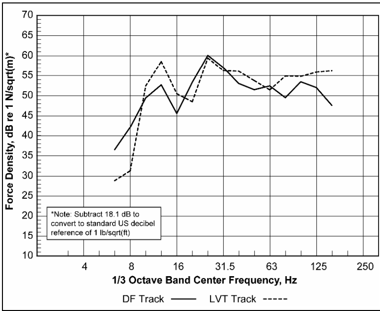
Fig. 11. Measured force density for direct fixation and LVT track, SFO Airport subway.
