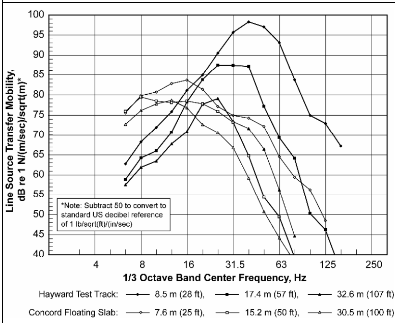
Fig. 4. Line source transfer mobilities measured at the Hayward test track and Concord floating slab test sites.
