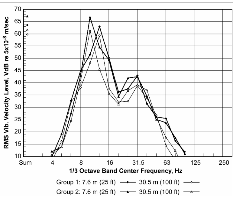
Fig. 10. Averages for two groups of trains at SFO Airport extension floating slab section.
