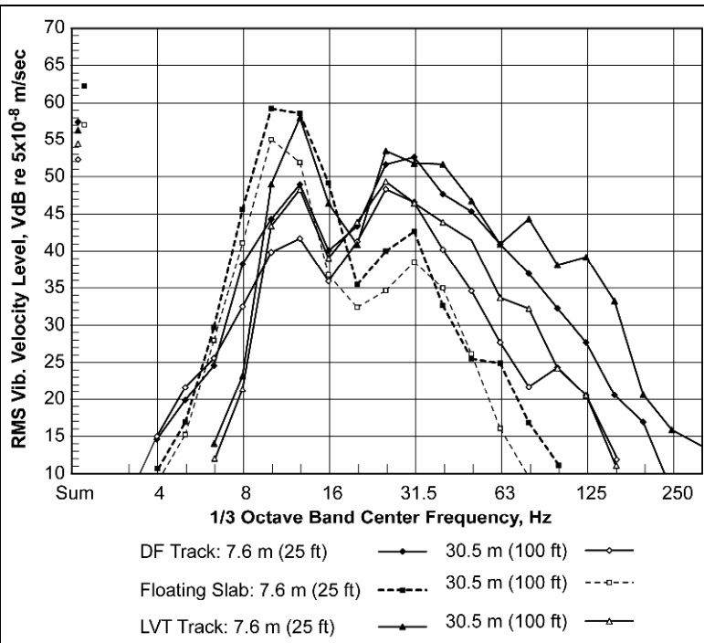
Fig. 9. Average vibration velocity levels measured at the ground surface above the San Francisco Airport Extension subway. All measurements were in the same general area of South San Francisco. Trains speeds are typically 65 mph in this area.
