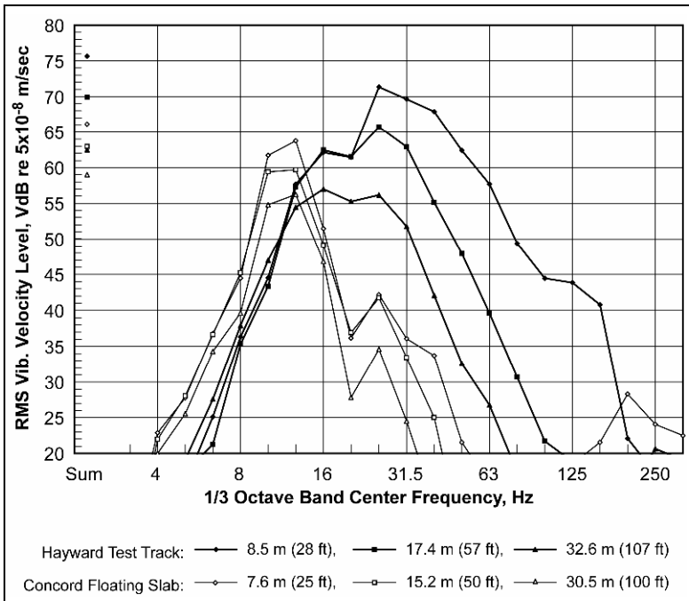
Fig. 3. Average vibration levels measured at Hayward Test Track and Concord floating slab. Average train speed was 65 mph at for both sites.
