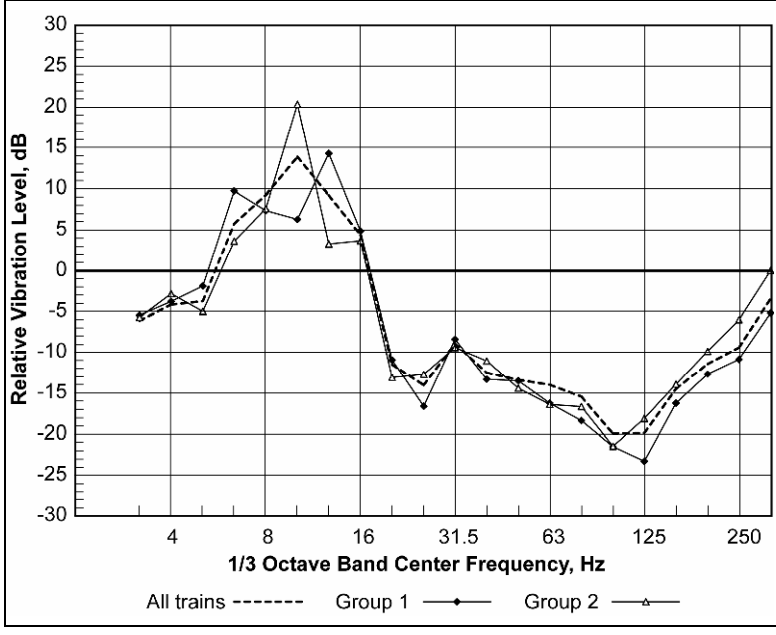
Fig. 12. Comparison of train vibration from direct fixation and floating slab test sections, SFO Airport subway. Shown are the average differences of floating slab vibration minus direct fixation vibration (a negative number implies an improvement by the floating slab).
