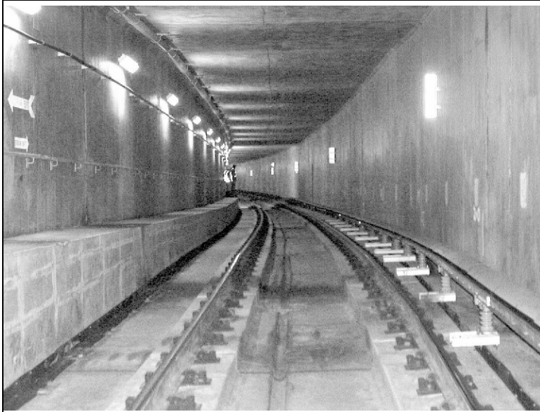
Fig. 8. Photograph of continuous floating slab track section in the San Francisco Airport Extension subway. Because there are no gaps between the floating slab and the subway invert larger than a few inches, impact testing from the invert to the surface was not feasible for this section of track.
